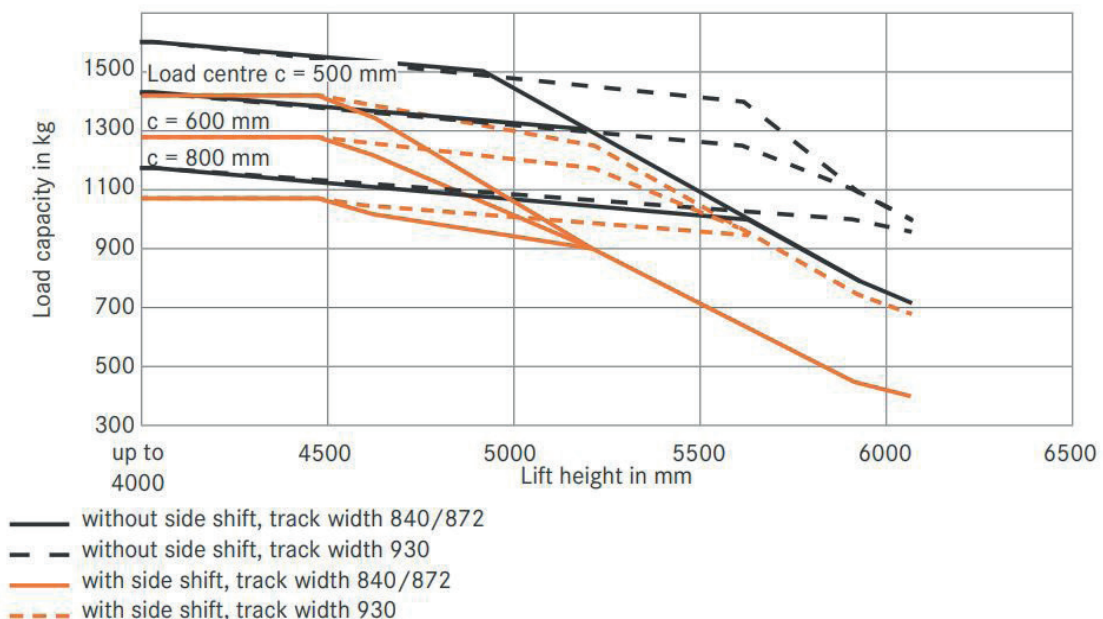
RX 50-16 triplex mast, Superelastic tyres
